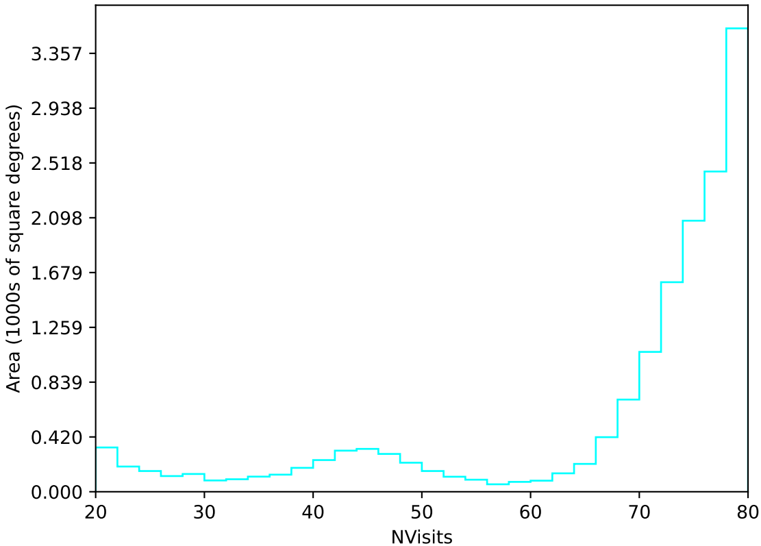
internal_u_expt38_nscale1.5v3.4_10yrs All sky u band: NVisits
