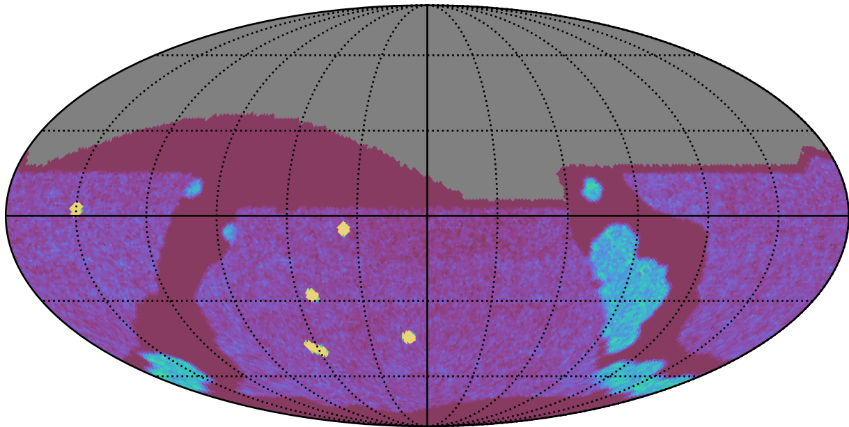
internal_u_expt38_nscale1.5v3.4_10yrs All sky g band: NVisits
