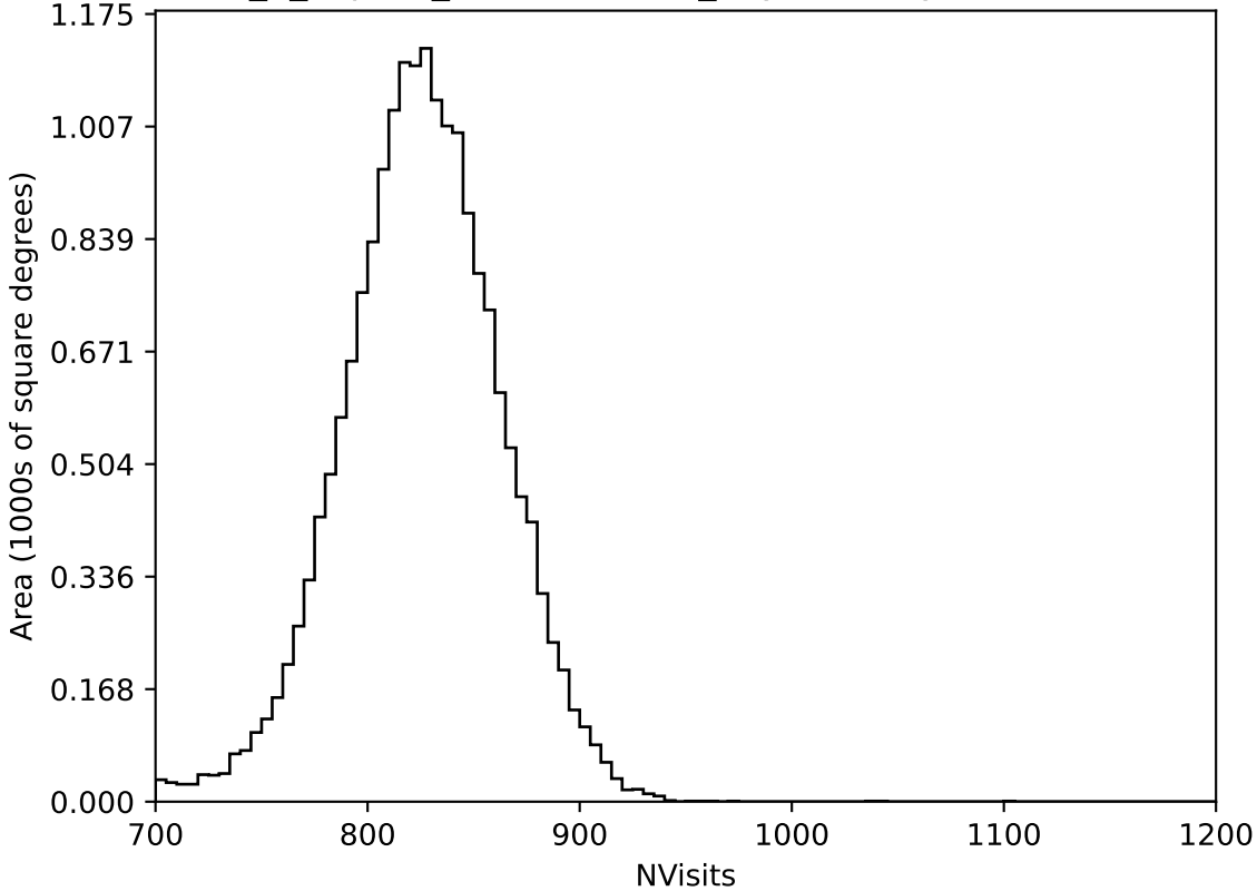
internal_u_expt38_nscale1.5v3.4_10yrs All sky all bands: NVisits
