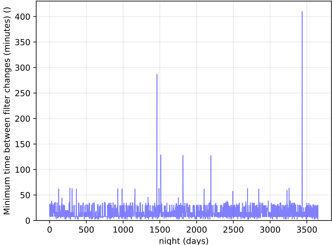
internal_u_expt38_nscale1.5v3.4_10yrs Per Night: Minimum time between filter changes (minutes)
