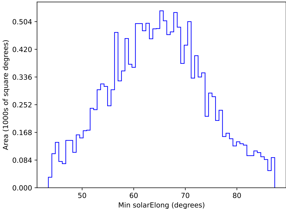
internal_u_expt38_nscale1.5v3.4_10yrs WFD y band: Min solarElong
