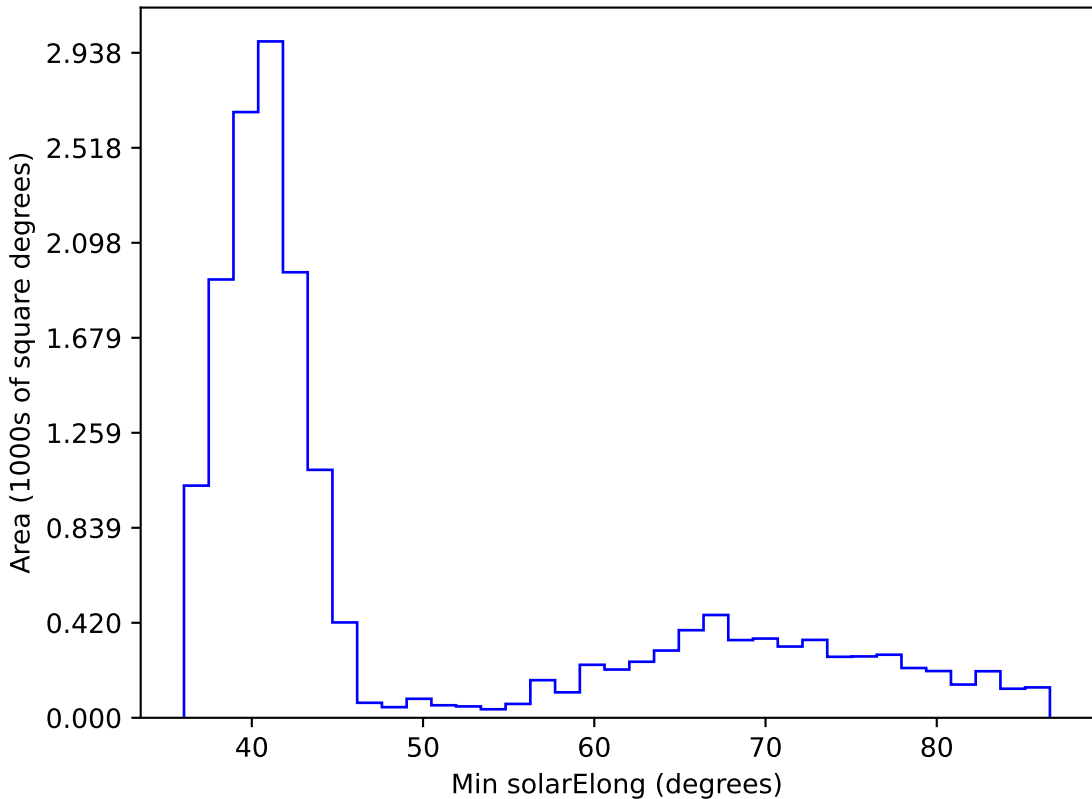
internal_u_expt38_nscale1.5v3.4_10yrs WFD i band: Min solarElong
