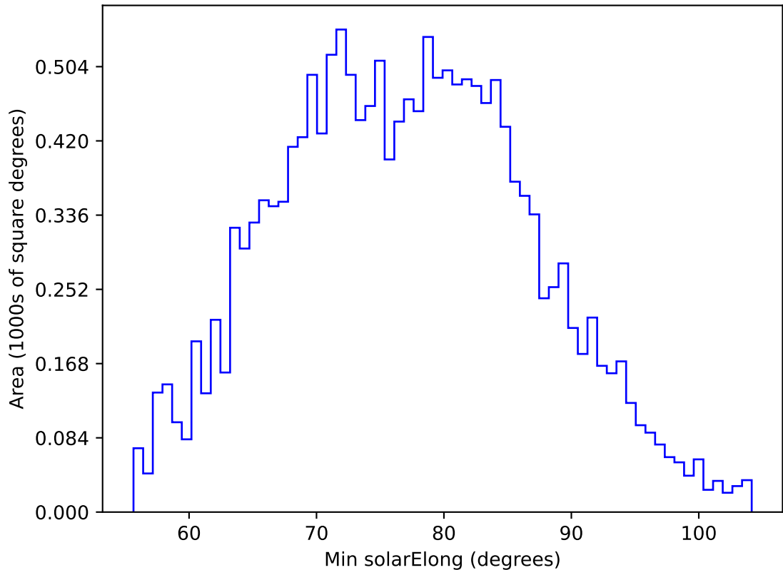
internal_u_expt38_nscale1.5v3.4_10yrs WFD g band: Min solarElong
