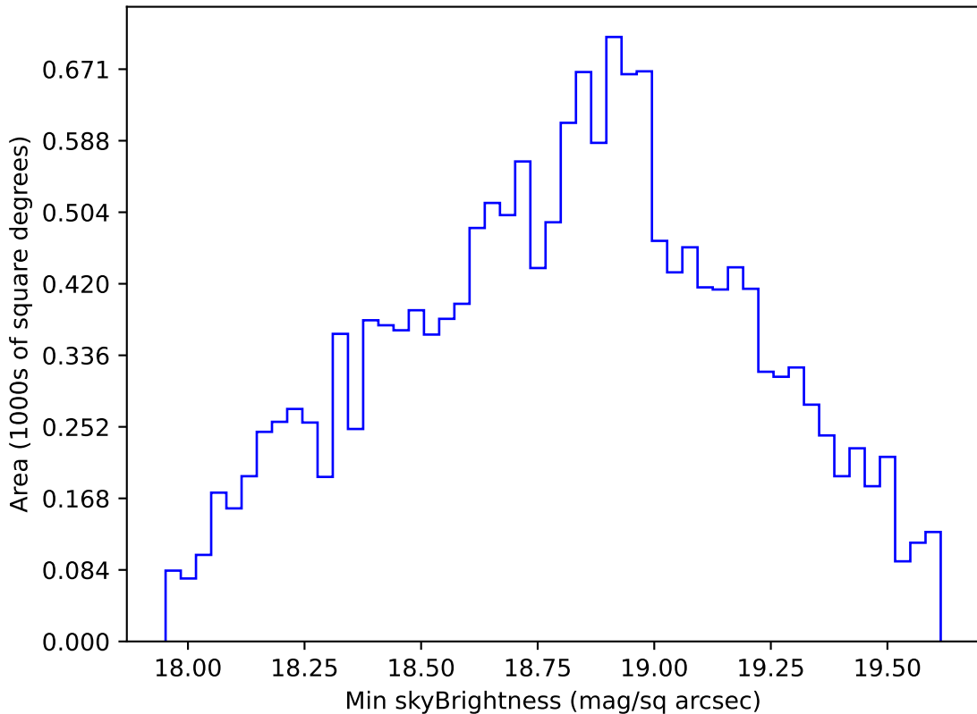
internal_u_expt38_nscale1.5v3.4_10yrs WFD r band: Min skyBrightness
