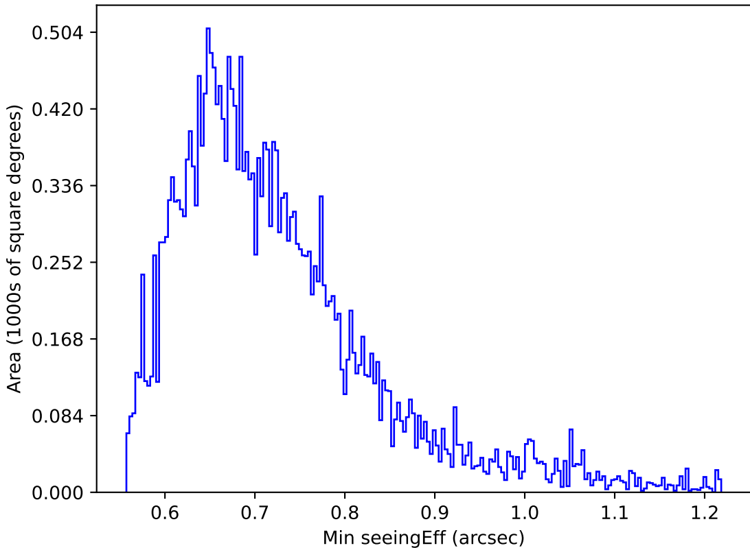
internal_u_expt38_nscale1.5v3.4_10yrs Yr 1 z band: Min seeingEff
