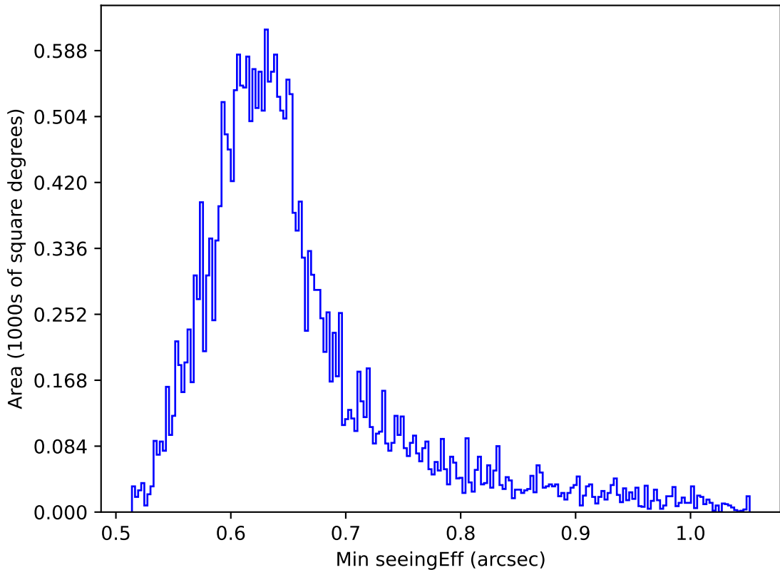
internal_u_expt38_nscale1.5v3.4_10yrs Yr 1 all bands: Min seeingEff
