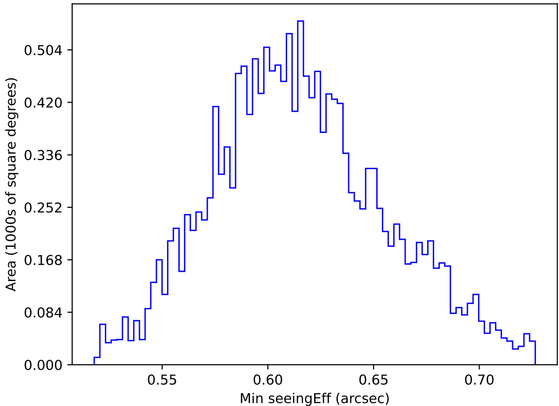
internal_u_expt38_nscale1.5v3.4_10yrs WFD z band: Min seeingEff
