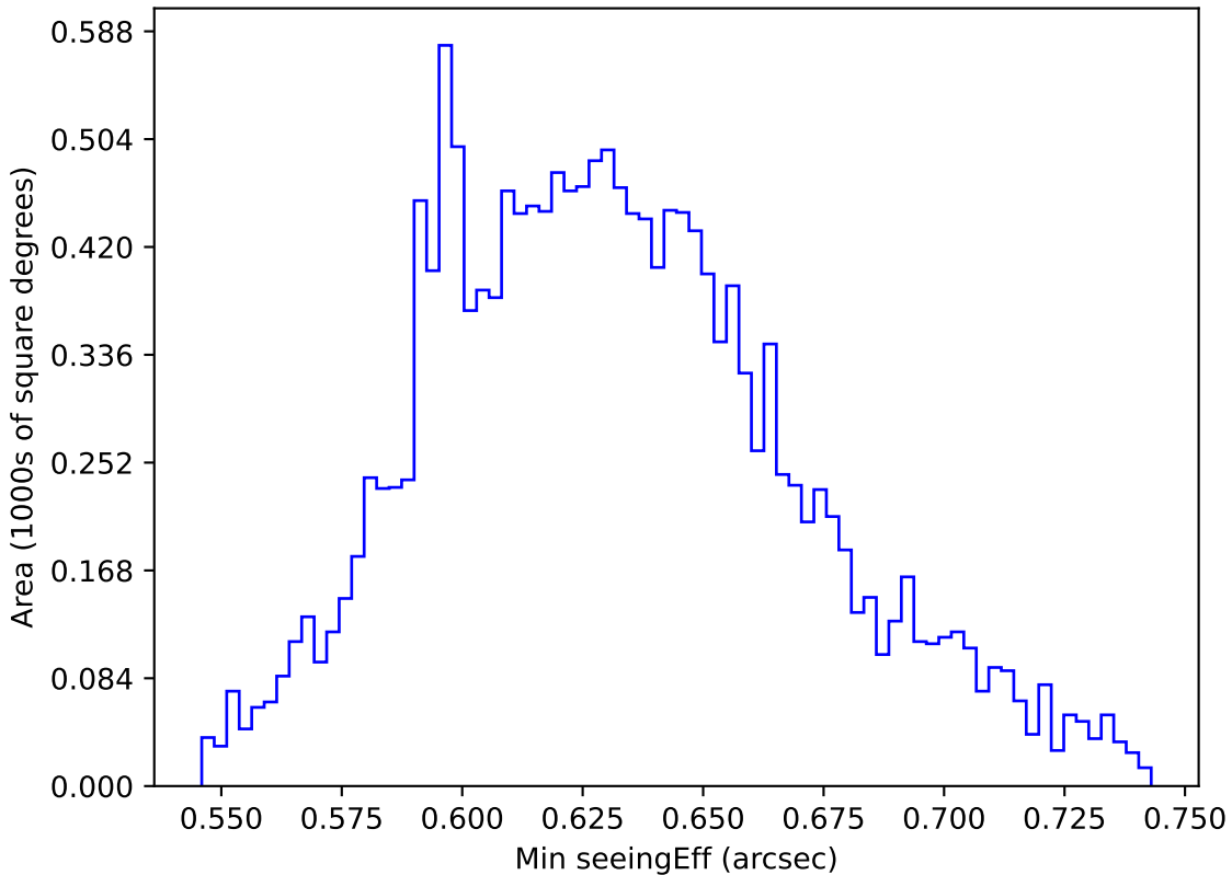
internal_u_expt38_nscale1.5v3.4_10yrs WFD y band: Min seeingEff
