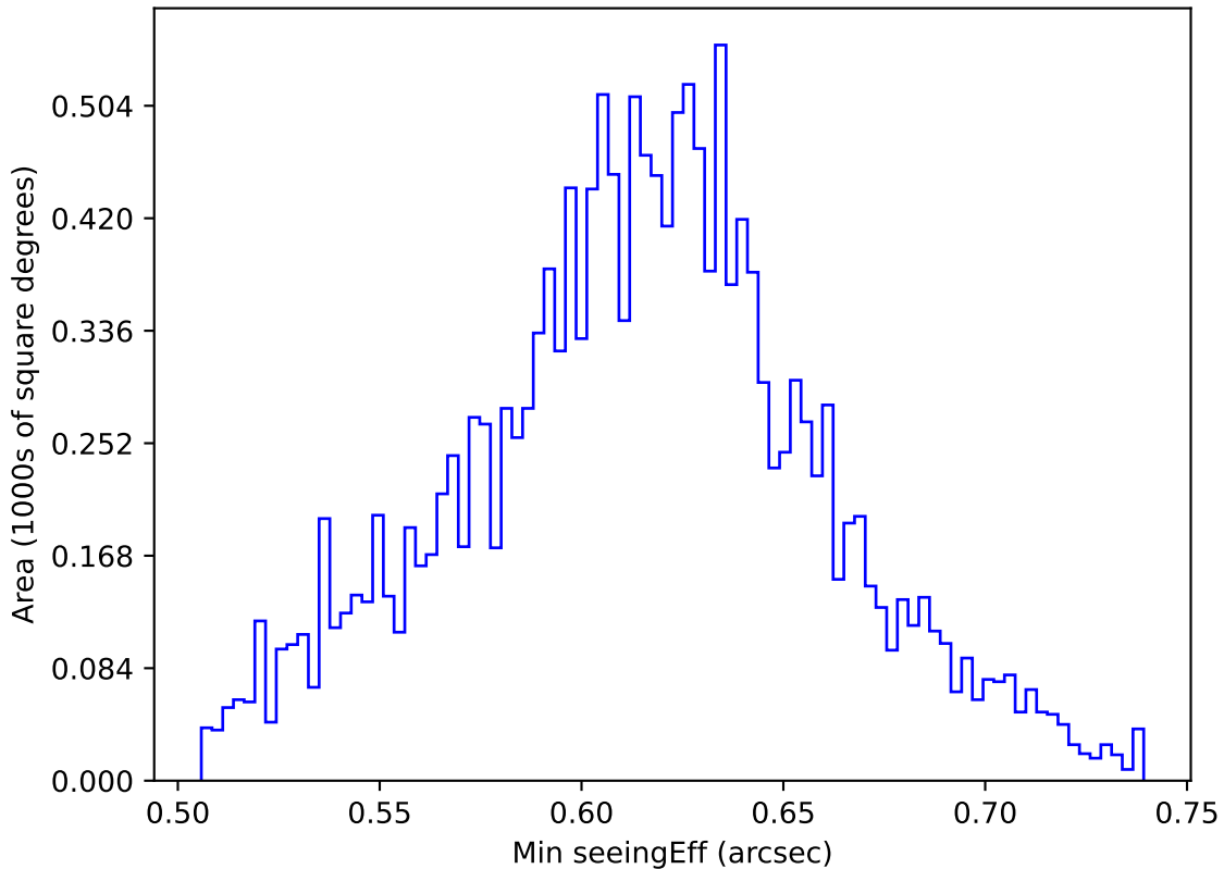
internal_u_expt38_nscale1.5v3.4_10yrs WFD r band: Min seeingEff
