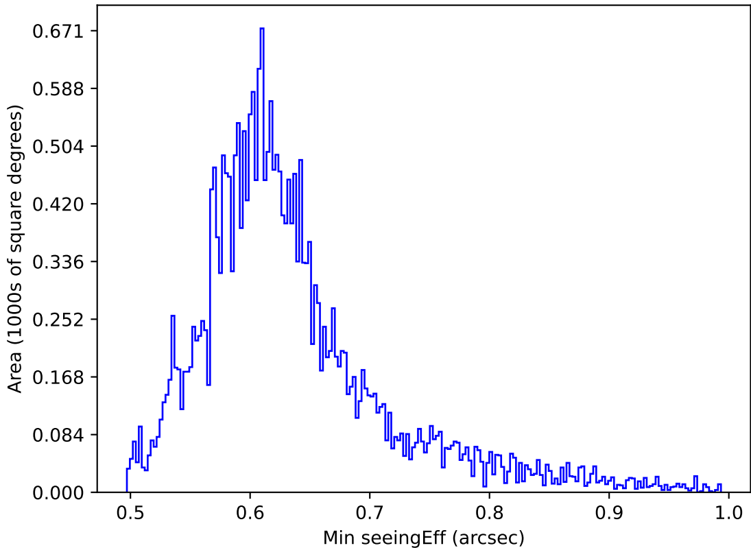
internal_u_expt38_nscale1.5v3.4_10yrs All sky i band: Min seeingEff
