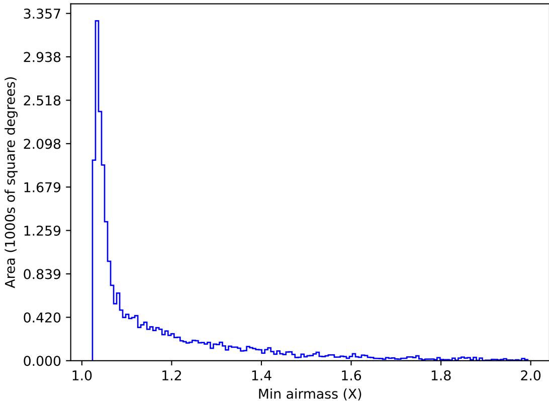
internal_u_expt38_nscale1.5v3.4_10yrs Yr 1 i band: Min airmass
