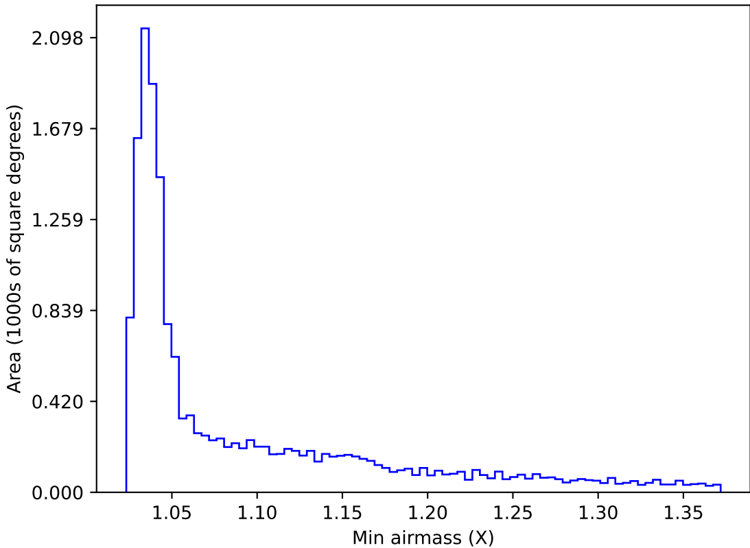
internal_u_expt38_nscale1.5v3.4_10yrs WFD u band: Min airmass
