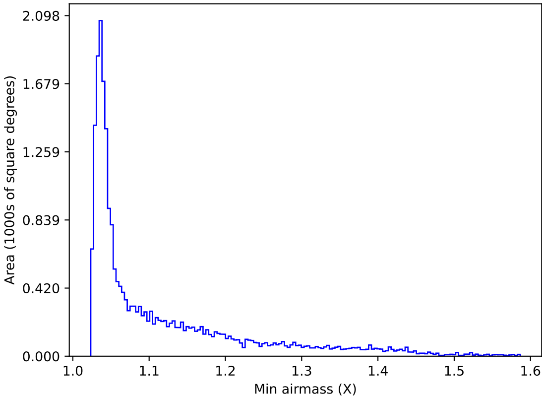
internal_u_expt38_nscale1.5v3.4_10yrs All sky u band: Min airmass
