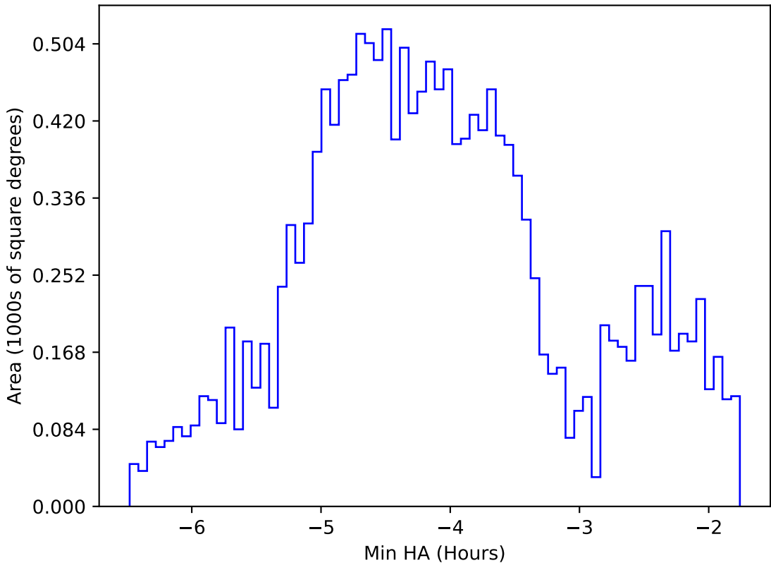
internal_u_expt38_nscale1.5v3.4_10yrs WFD g band: Min HA
