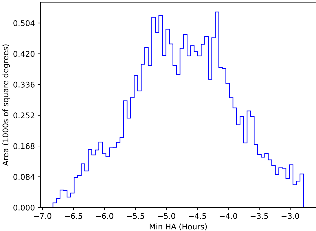
internal_u_expt38_nscale1.5v3.4_10yrs WFD all bands: Min HA
