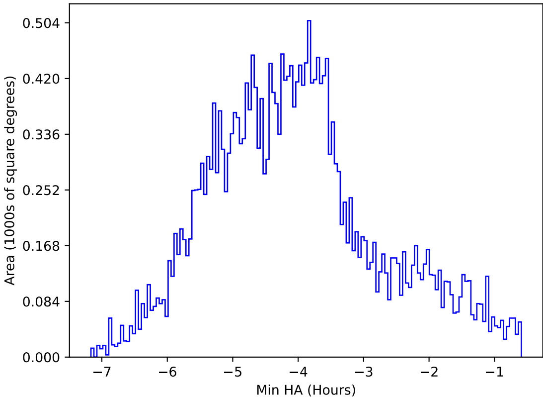
internal_u_expt38_nscale1.5v3.4_10yrs All sky z band: Min HA
