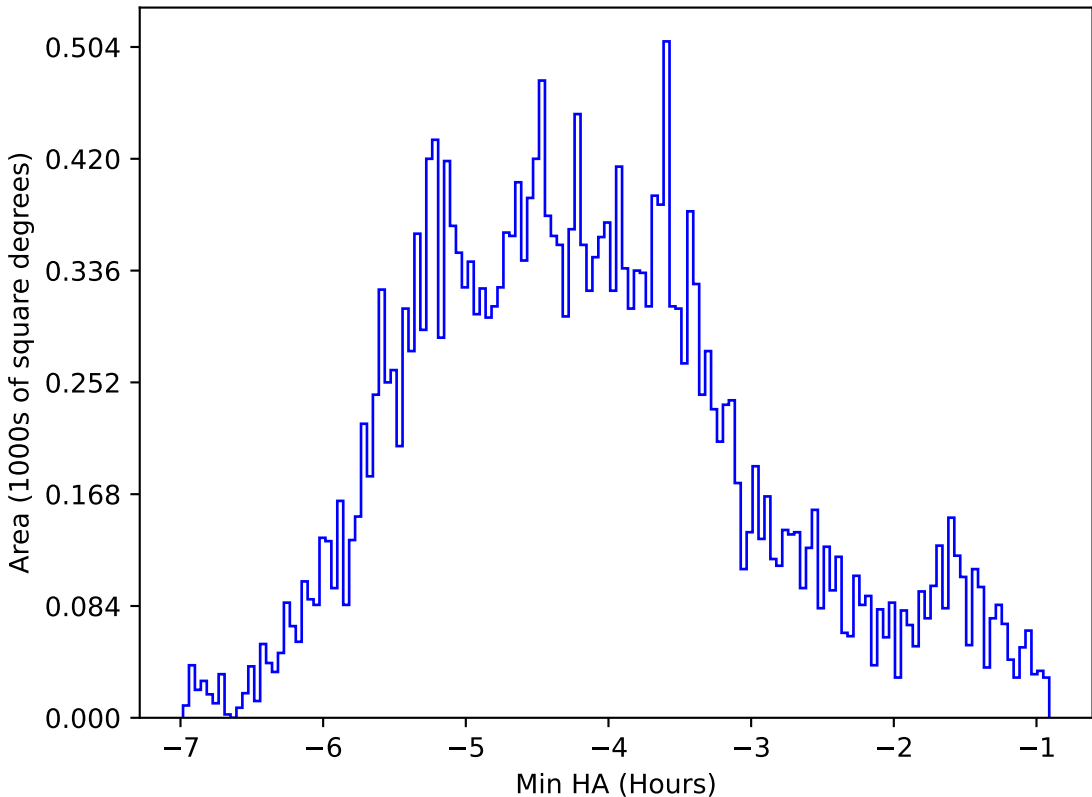
internal_u_expt38_nscale1.5v3.4_10yrs All sky r band: Min HA
