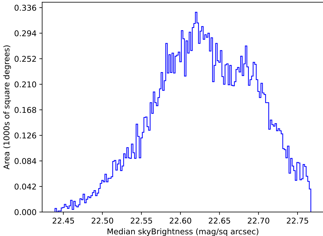
internal_u_expt38_nscale1.5v3.4_10yrs Yr 1 u band: Median skyBrightness
