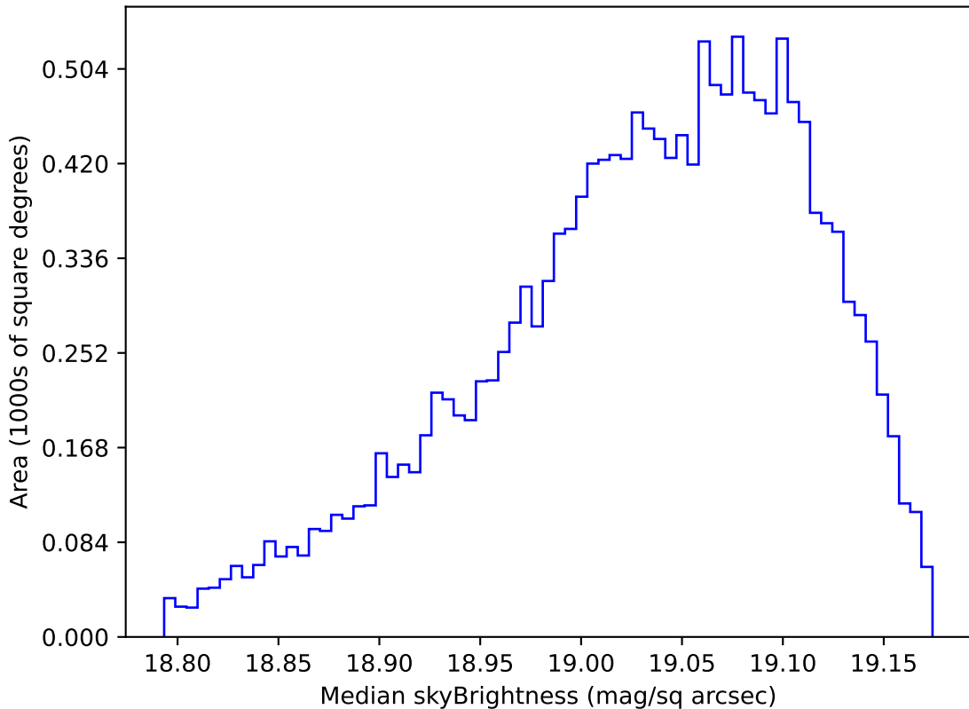
internal_u_expt38_nscale1.5v3.4_10yrs WFD z band: Median skyBrightness
