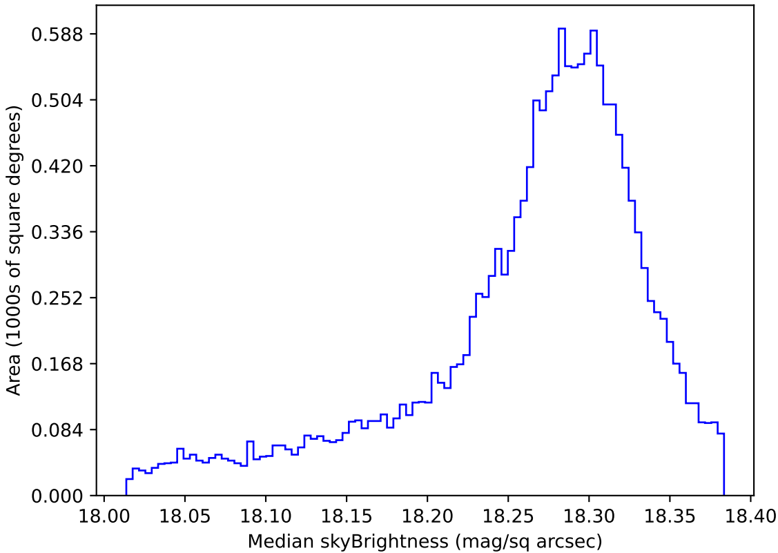
internal_u_expt38_nscale1.5v3.4_10yrs WFD y band: Median skyBrightness
