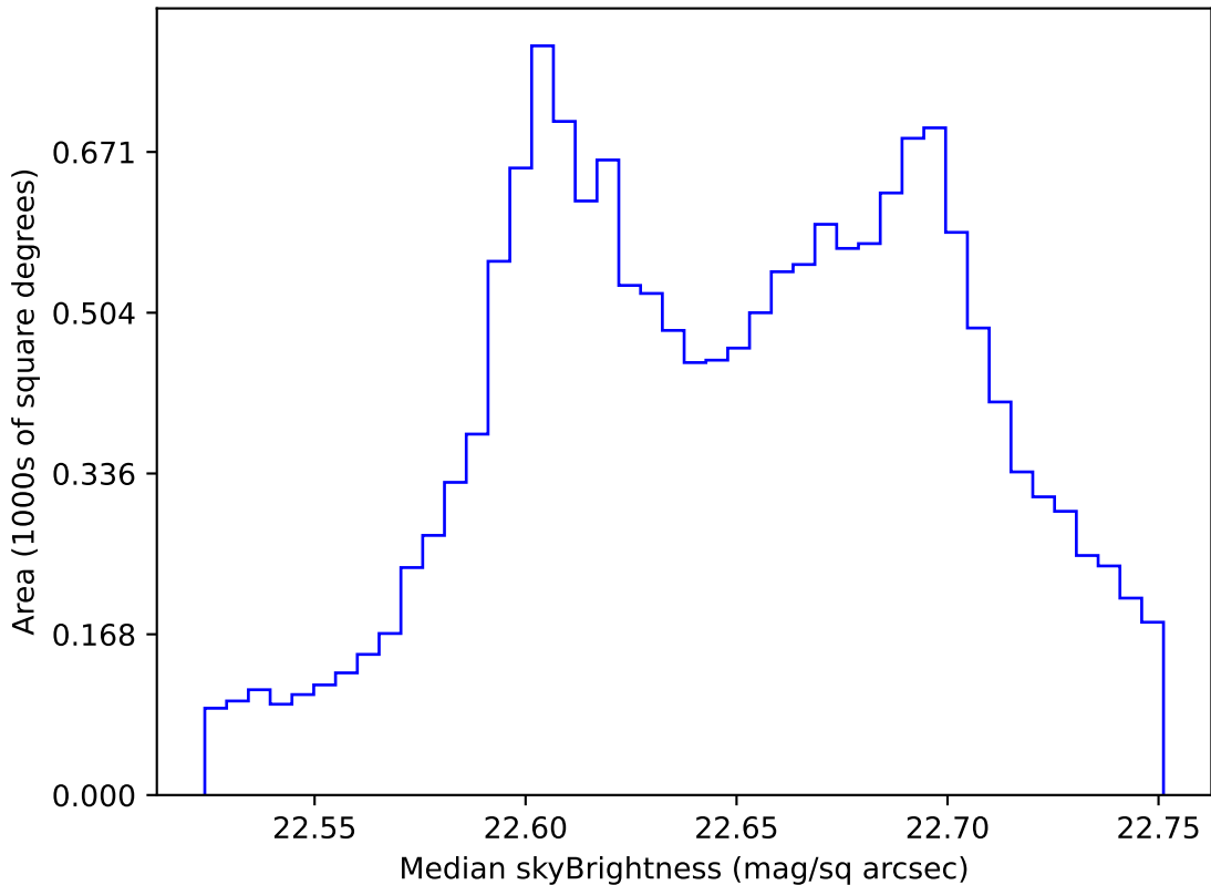
internal_u_expt38_nscale1.5v3.4_10yrs WFD u band: Median skyBrightness
