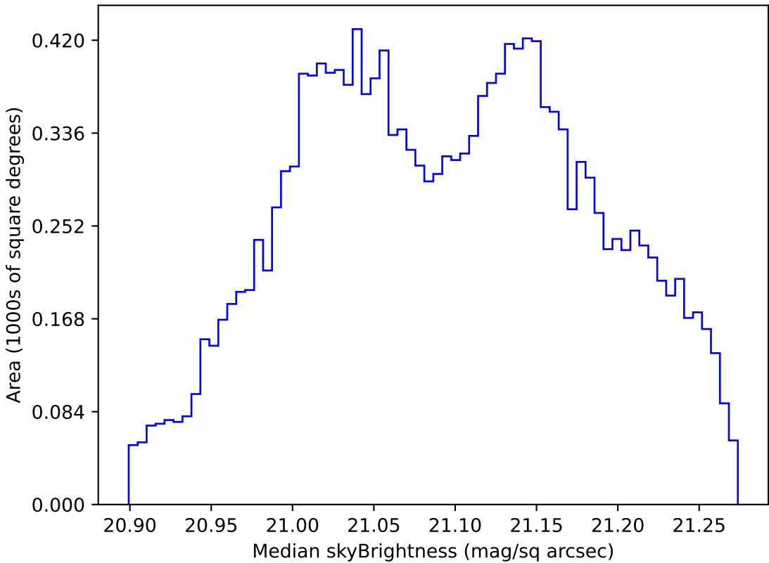
internal_u_expt38_nscale1.5v3.4_10yrs WFD r band: Median skyBrightness
