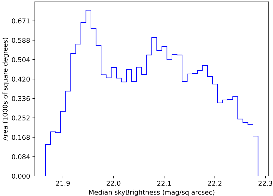
internal_u_expt38_nscale1.5v3.4_10yrs WFD g band: Median skyBrightness
