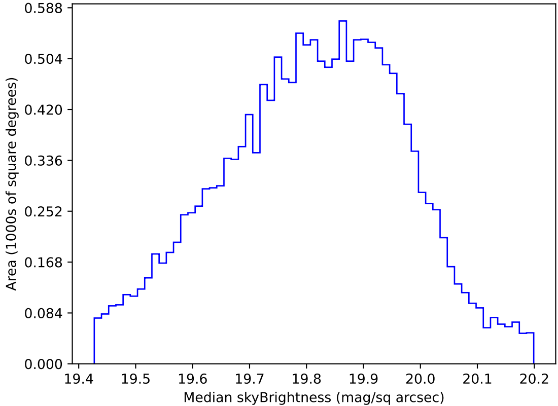
internal_u_expt38_nscale1.5v3.4_10yrs WFD all bands: Median skyBrightness
