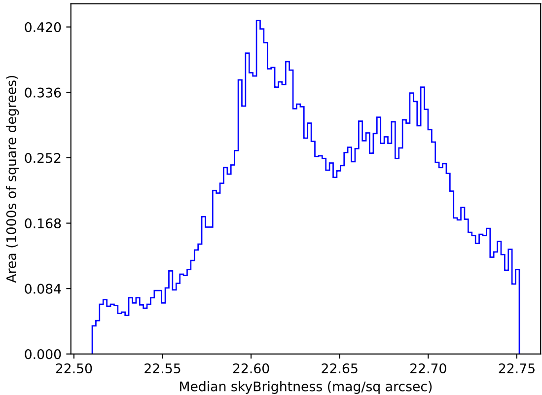
internal_u_expt38_nscale1.5v3.4_10yrs All sky u band: Median skyBrightness
