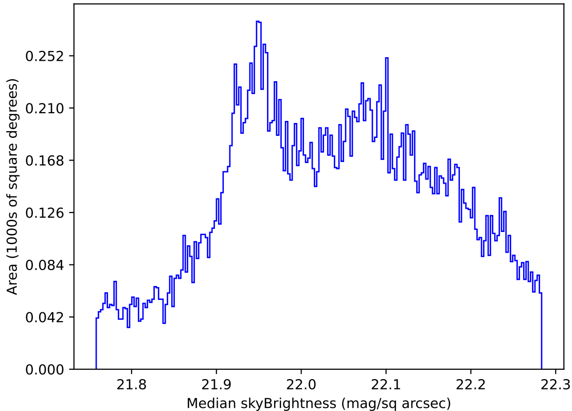
internal_u_expt38_nscale1.5v3.4_10yrs All sky g band: Median skyBrightness
