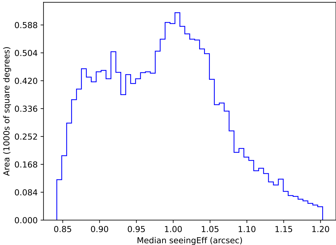
internal_u_expt38_nscale1.5v3.4_10yrs WFD i band: Median seeingEff
