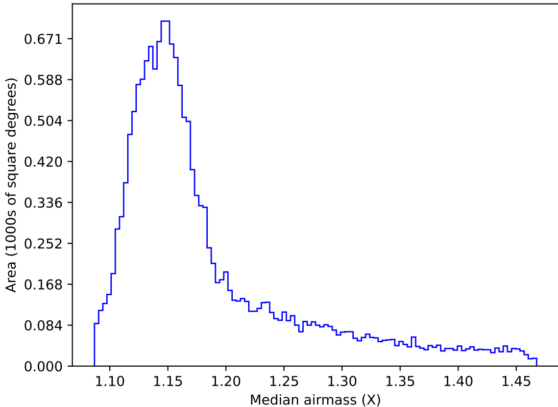
internal_u_expt38_nscale1.5v3.4_10yrs WFD z band: Median airmass
