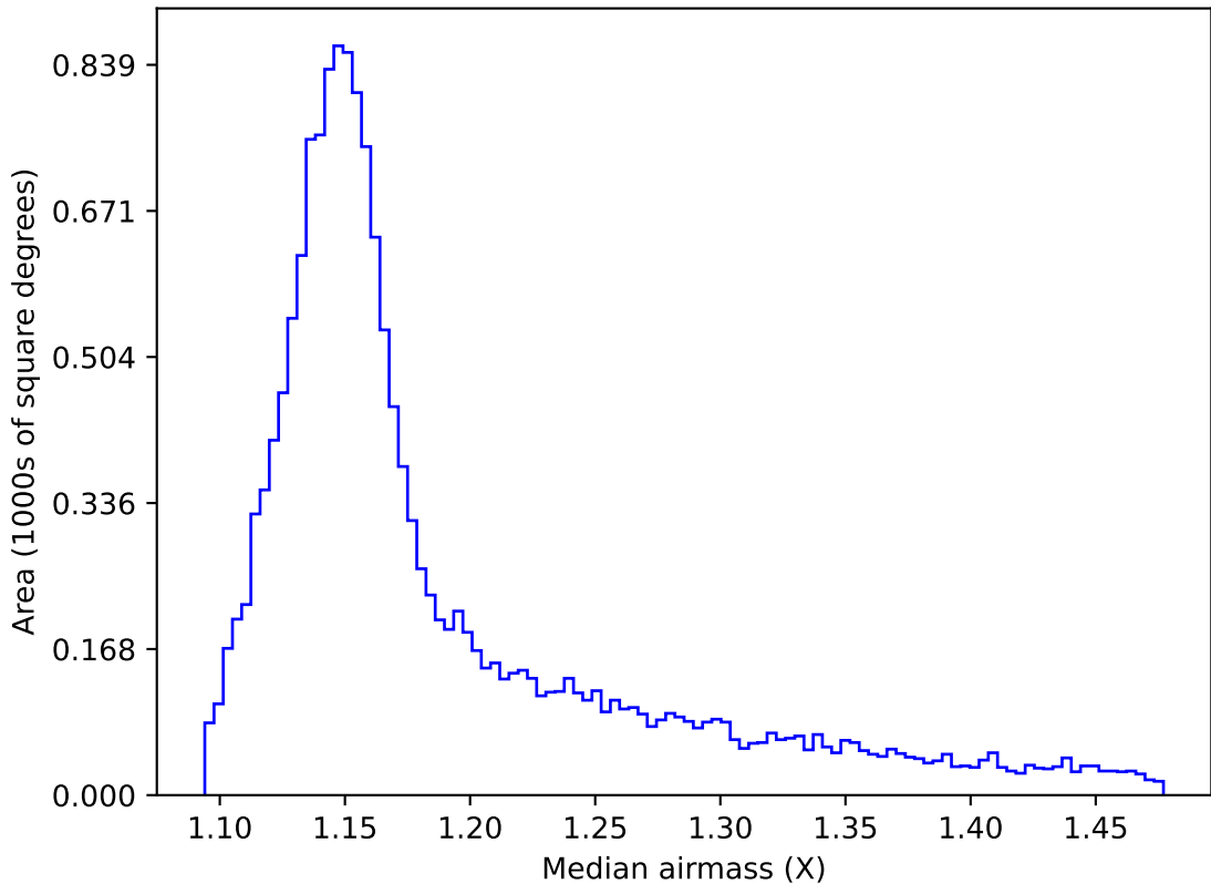
internal_u_expt38_nscale1.5v3.4_10yrs WFD y band: Median airmass
