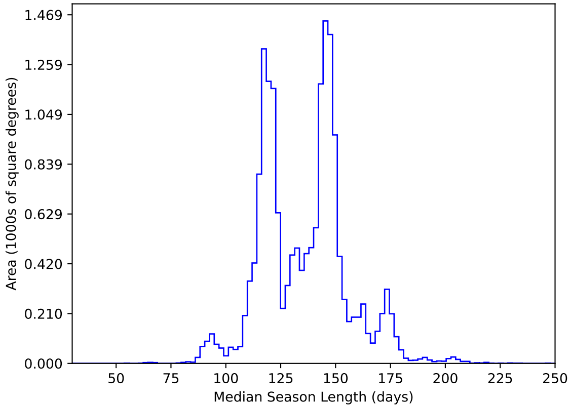
internal_u_expt38_nscale1.5v3.4_10yrs WFD y band: Median Season Length
