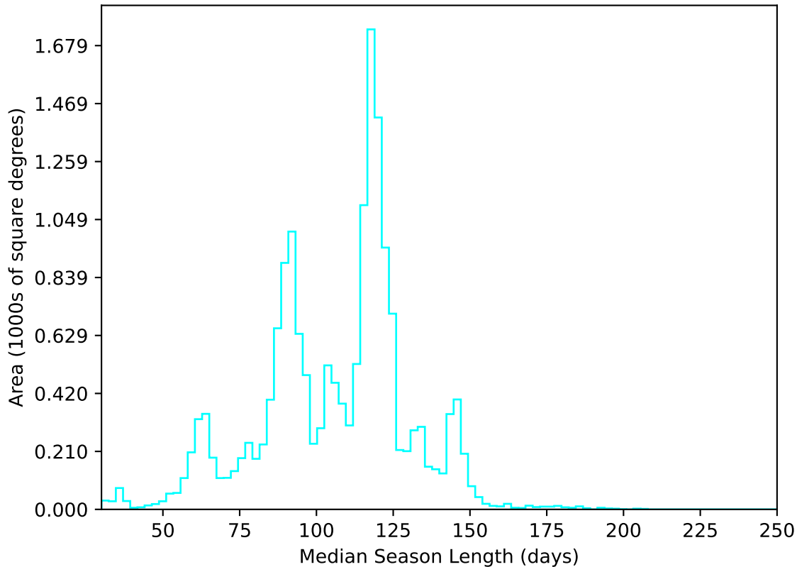
internal_u_expt38_nscale1.5v3.4_10yrs WFD u band: Median Season Length
