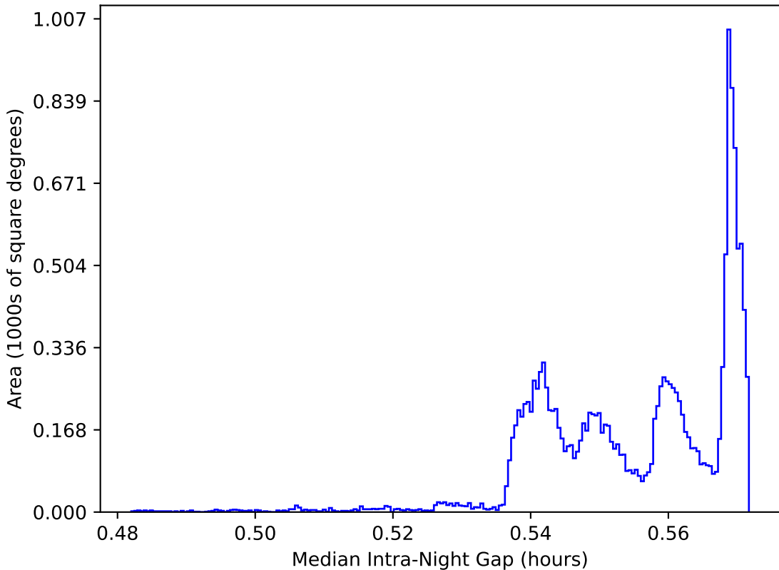
internal_u_expt38_nscale1.5v3.4_10yrs WFD: Median Intra-Night Gap
