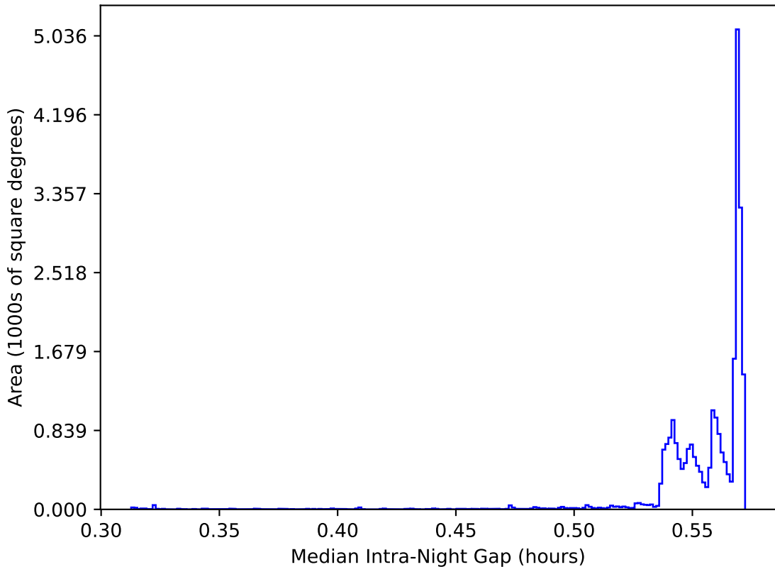
internal_u_expt38_nscale1.5v3.4_10yrs All sky: Median Intra-Night Gap
