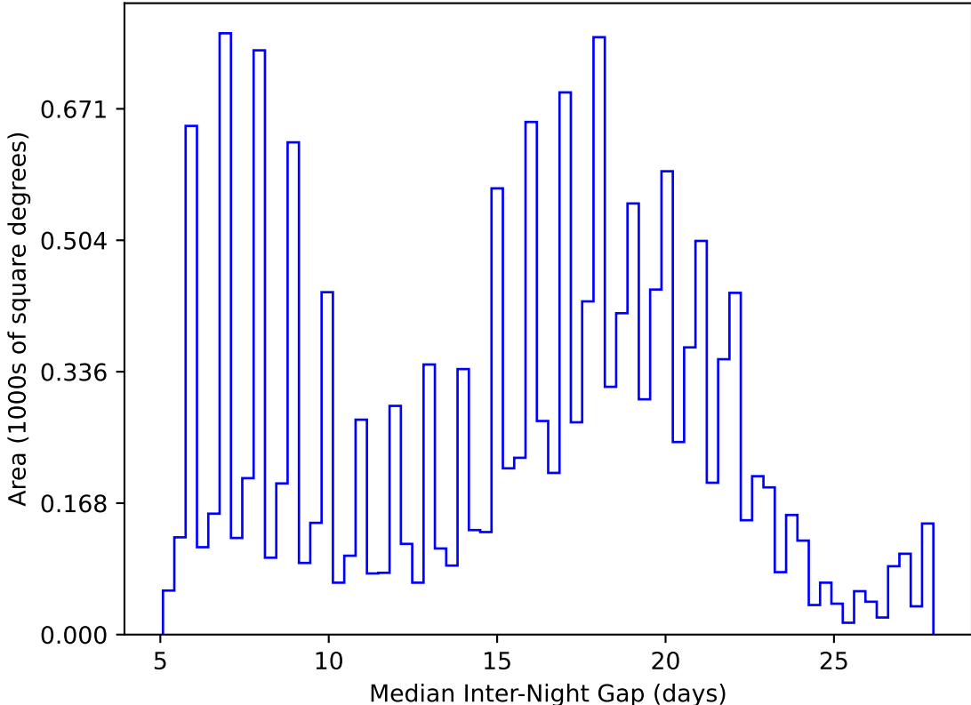
internal_u_expt38_nscale1.5v3.4_10yrs WFD y band: Median Inter-Night Gap
