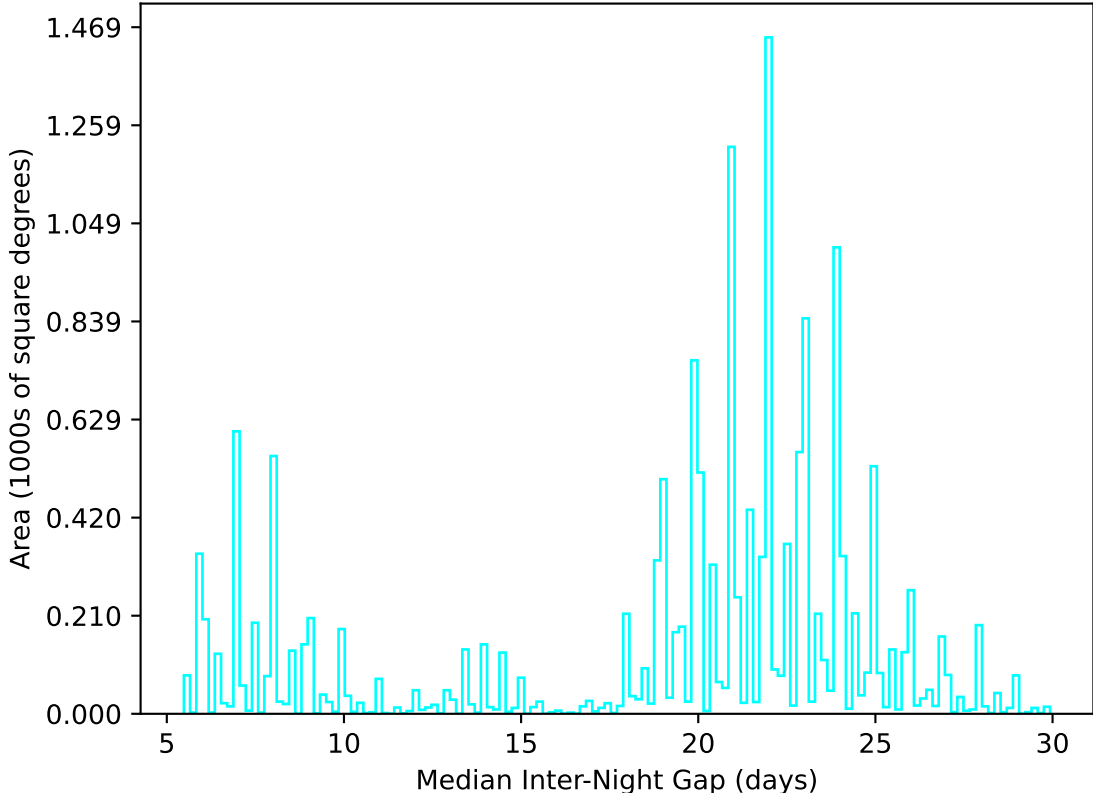
internal_u_expt38_nscale1.5v3.4_10yrs WFD u band: Median Inter-Night Gap
