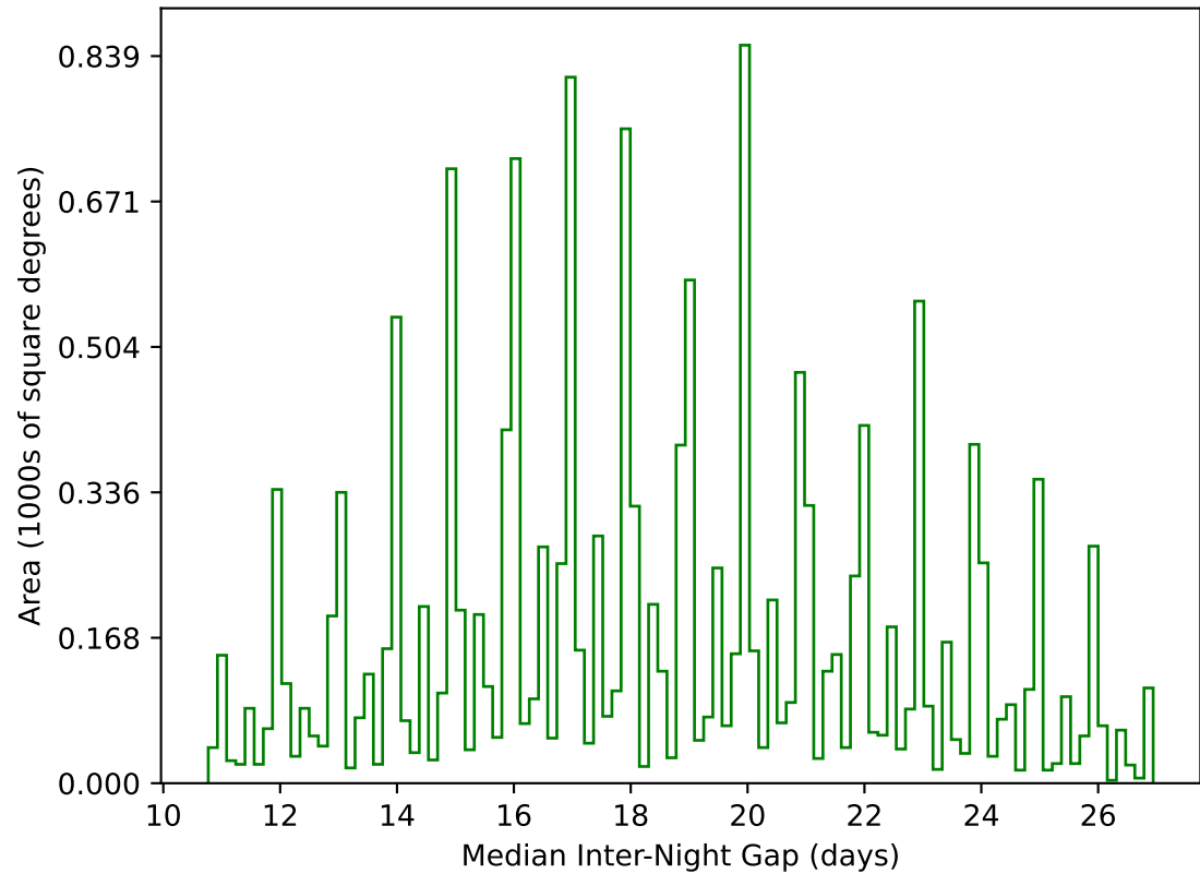
internal_u_expt38_nscale1.5v3.4_10yrs WFD g band: Median Inter-Night Gap
