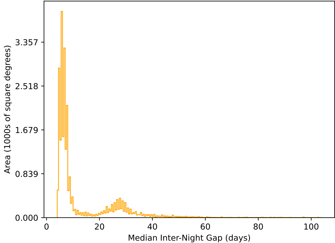
internal_u_expt38_nscale1.5v3.4_10yrs All sky r band: Median Inter-Night Gap
