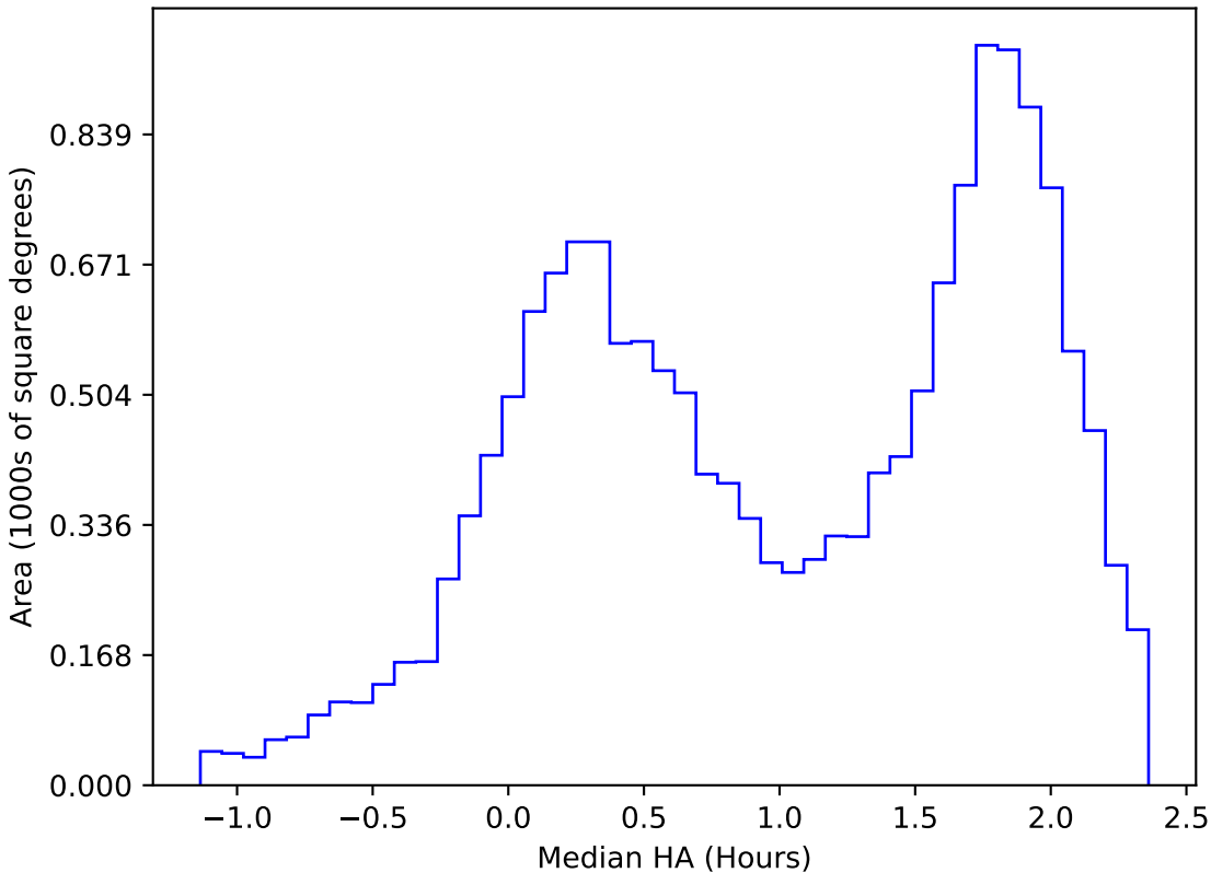
internal_u_expt38_nscale1.5v3.4_10yrs WFD u band: Median HA
