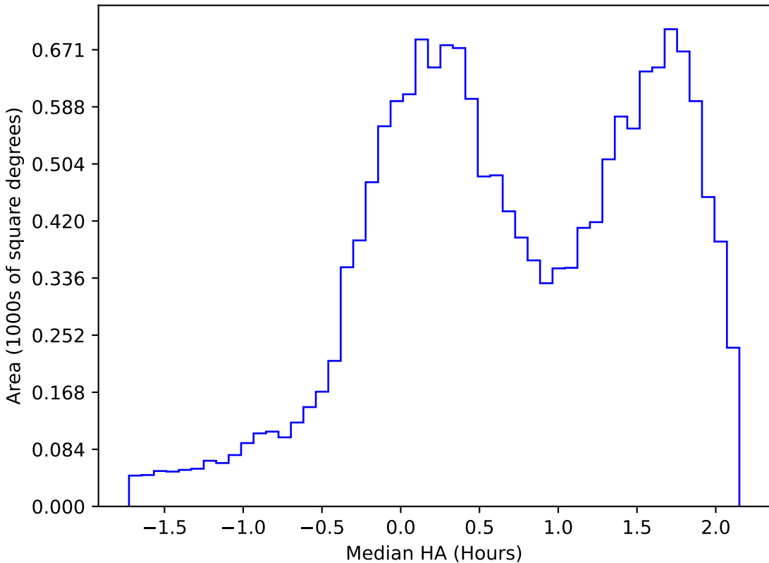
internal_u_expt38_nscale1.5v3.4_10yrs WFD g band: Median HA
