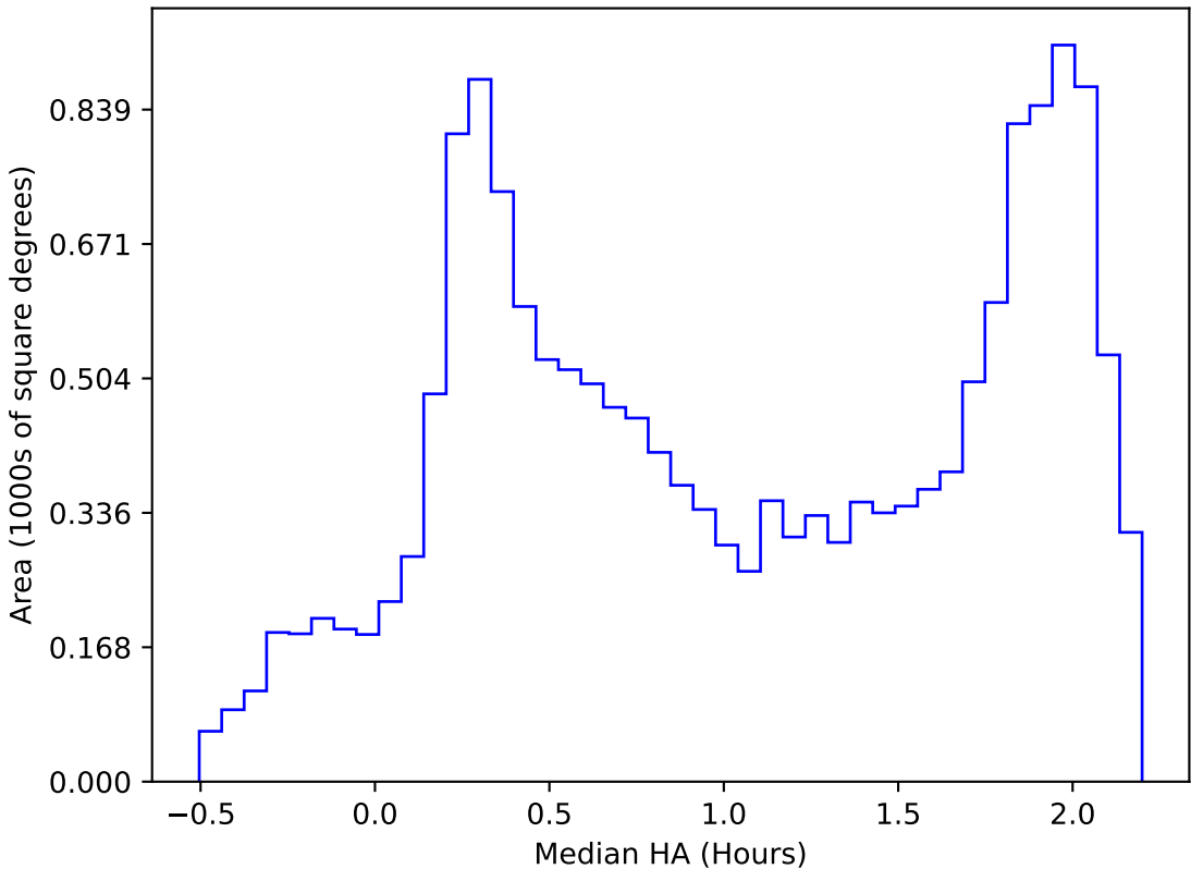
internal_u_expt38_nscale1.5v3.4_10yrs WFD all bands: Median HA
