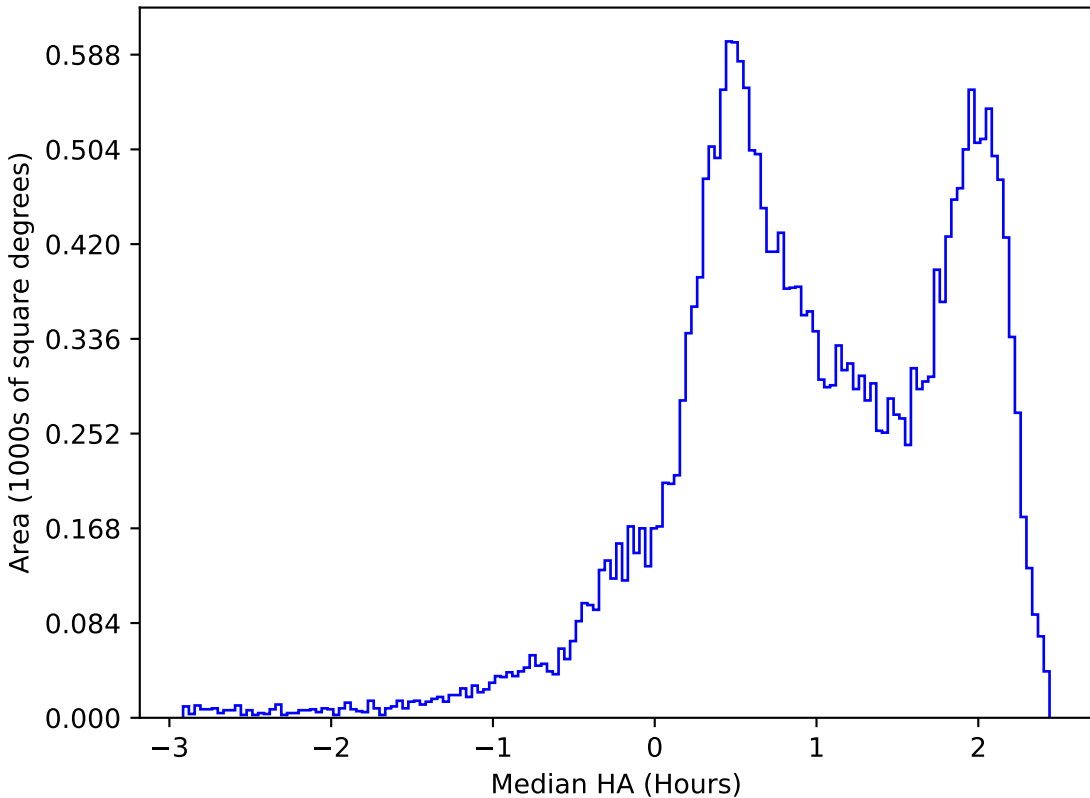
internal_u_expt38_nscale1.5v3.4_10yrs All sky z band: Median HA
