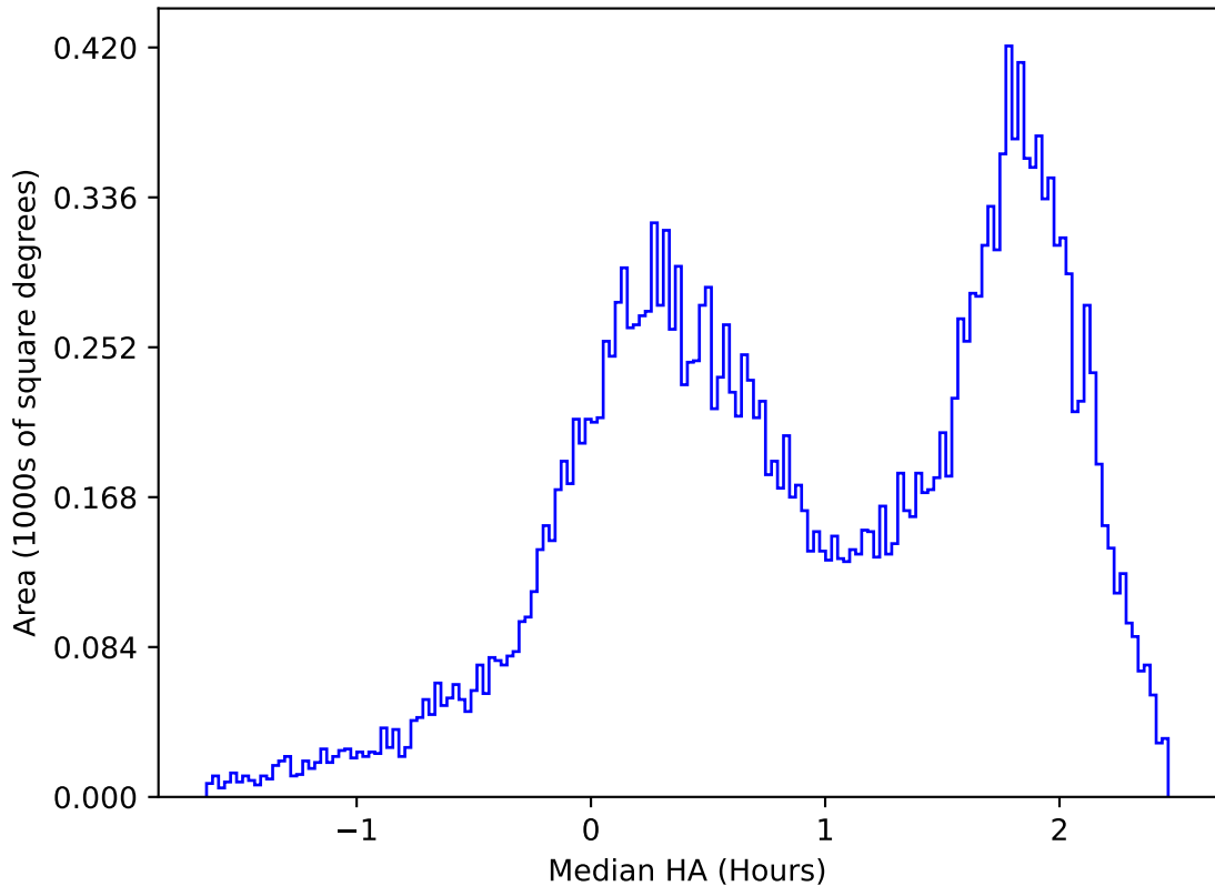
internal_u_expt38_nscale1.5v3.4_10yrs All sky u band: Median HA
