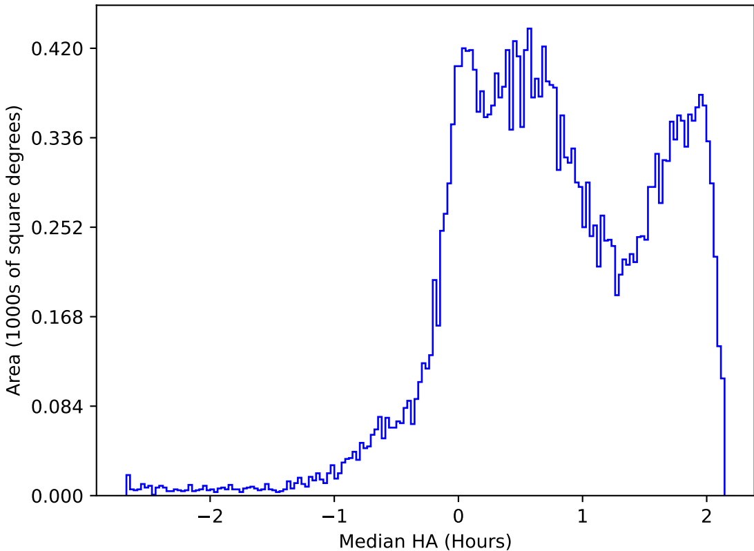
internal_u_expt38_nscale1.5v3.4_10yrs All sky r band: Median HA
