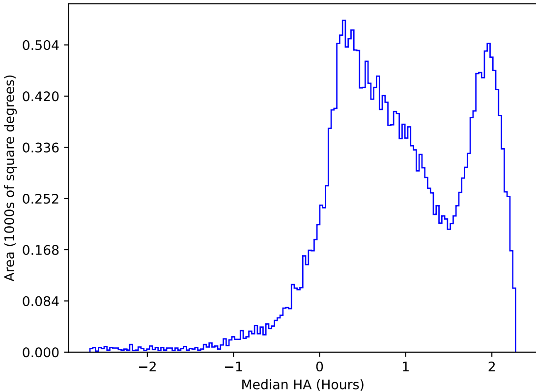
internal_u_expt38_nscale1.5v3.4_10yrs All sky i band: Median HA
