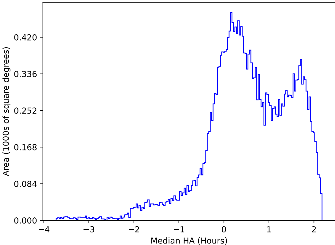
internal_u_expt38_nscale1.5v3.4_10yrs All sky g band: Median HA
