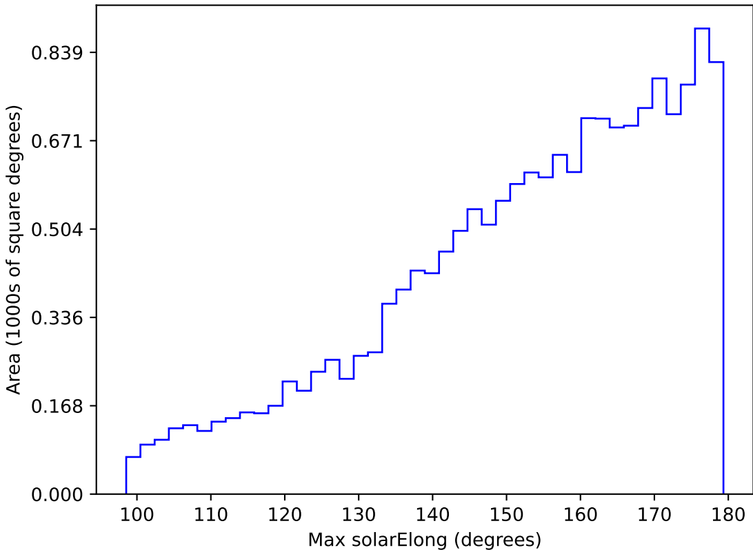
internal_u_expt38_nscale1.5v3.4_10yrs WFD y band: Max solarElong
